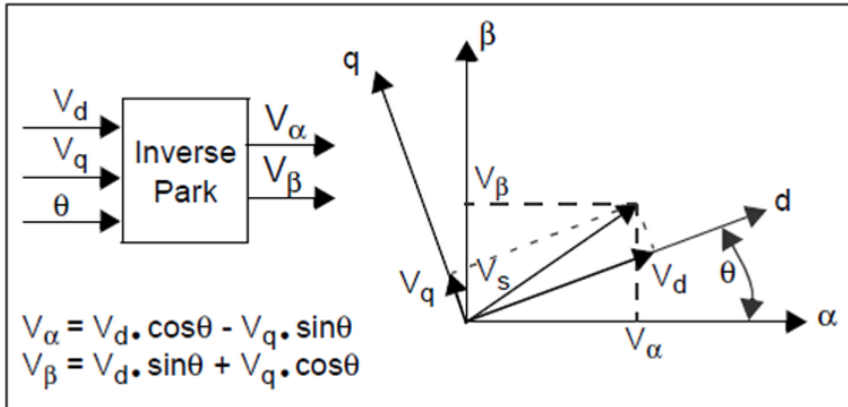
Figure 1-9. Inverse Park Transform
