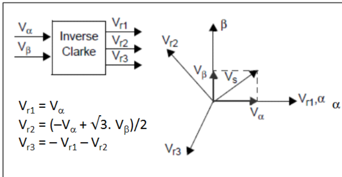
Figure 1-10. Inverse Clark Transform
