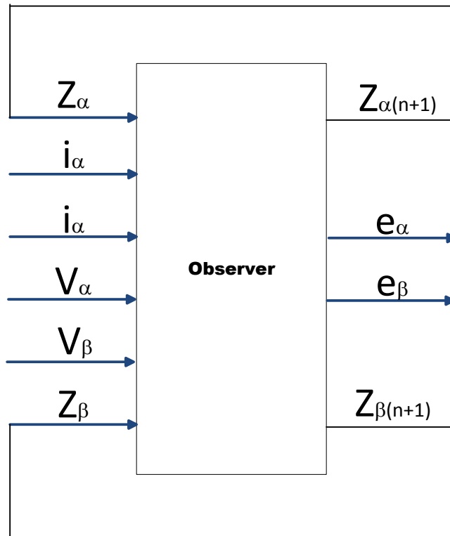
Figure 1-11. Reduced Order Luenberger Observer
